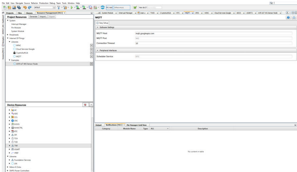
Figure 2-28. MQTT
