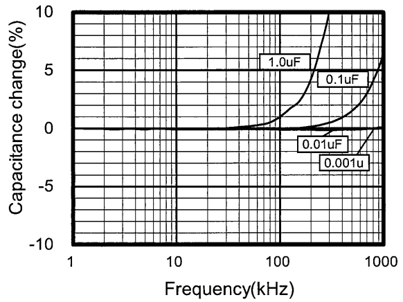
Frequency Characteristics
