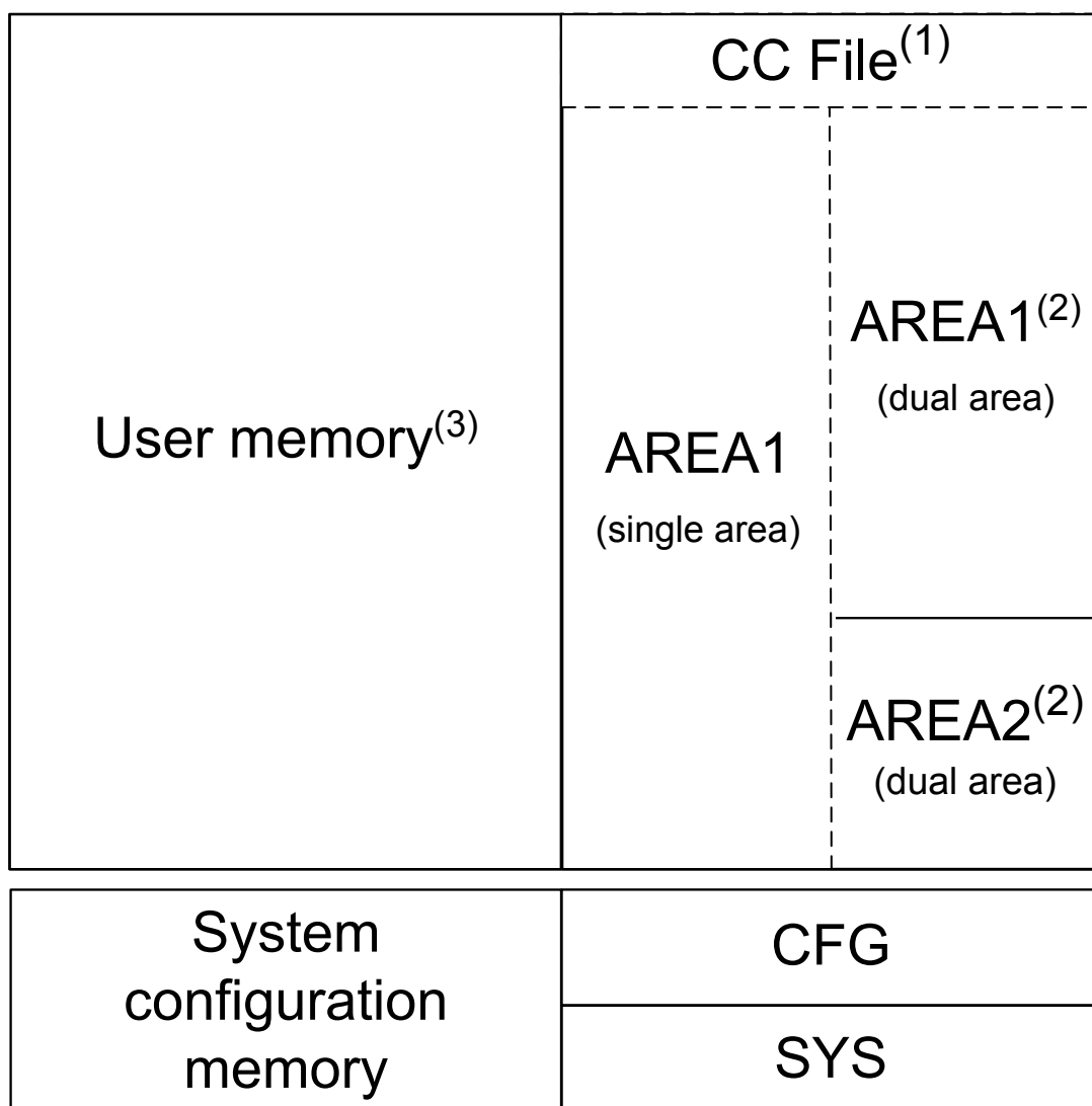
Figure 5. Memory organization
