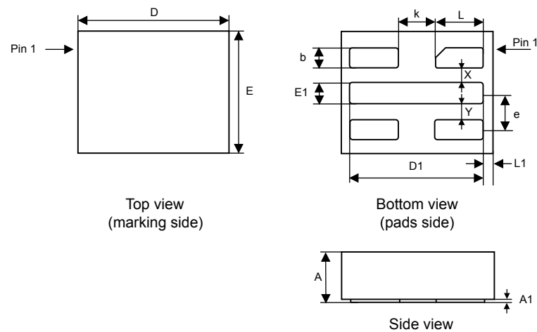
Figure 15. UFDFPN5 - Outline
