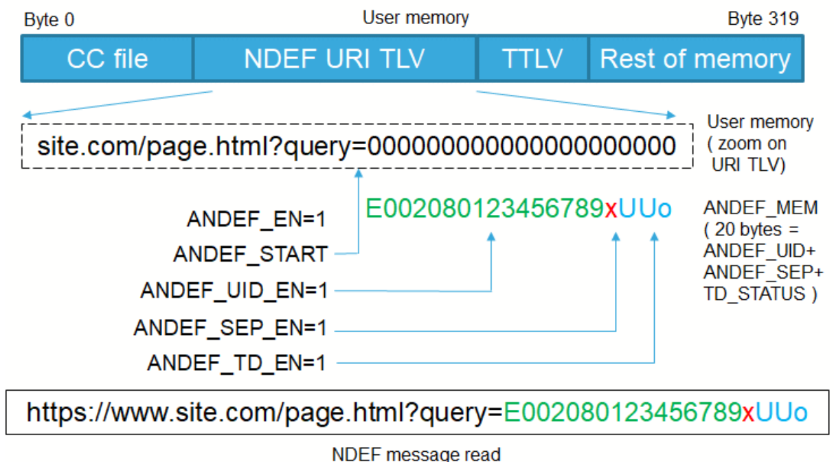
Figure 7. Example of augmented NDEF message on ST25TV02KC-T
