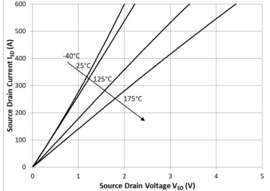
Figure 5 : 3rd quadrant characteristics ( V_{GS}=15V , t_p < 200\mu s ) 7
