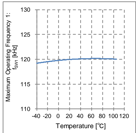
Figure 30. Maximum Operating Frequency 1 vs Temperature
