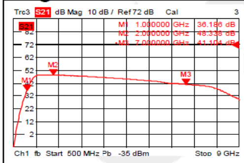
Gain @-45°C
