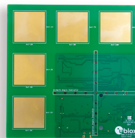
C211 antenna array board
