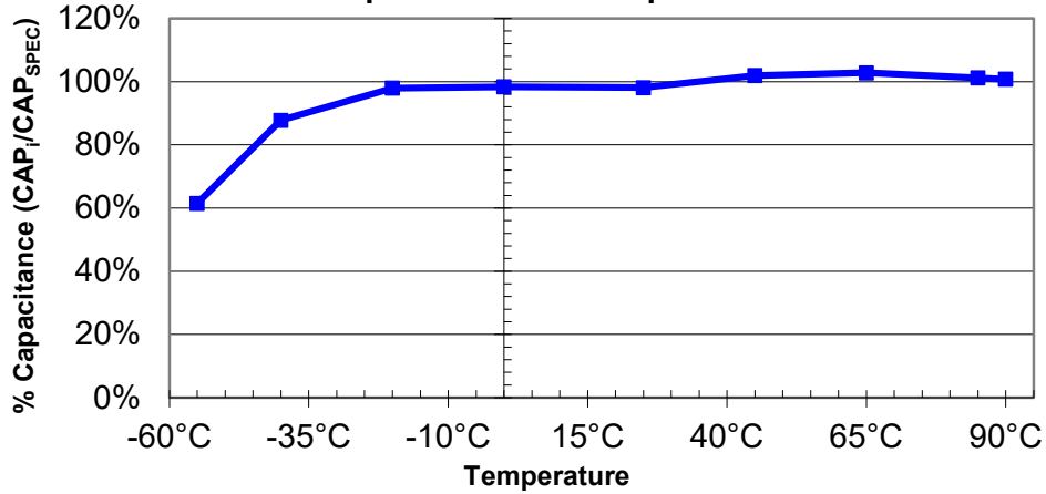
Capacitance vs. Temperature
