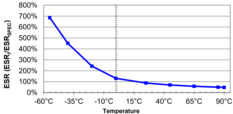
Equivalent Series Resistance vs. Temperature
