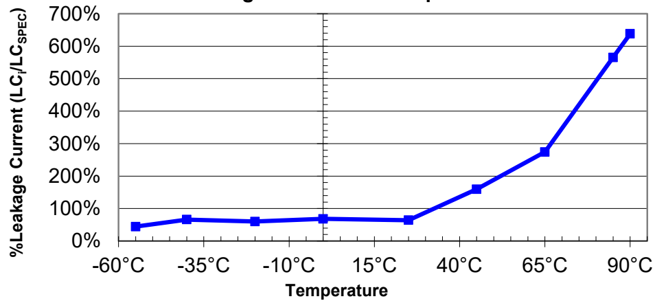
Leakage Current vs. Temperature
