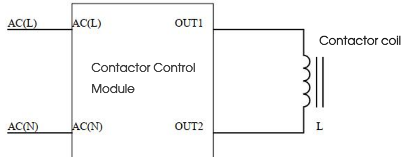
See Fig. 1 Typical application
