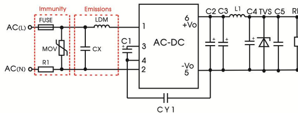
Application circuit 4
