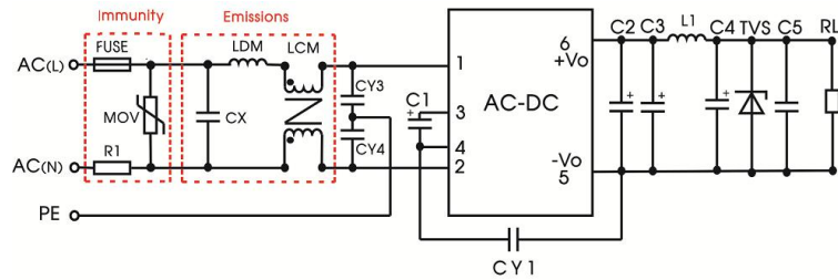
Application circuit 5
