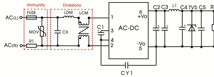
Application circuit 3
