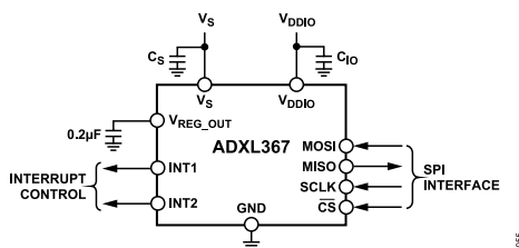
Figure 60. Recommended Bypass Capacitors
