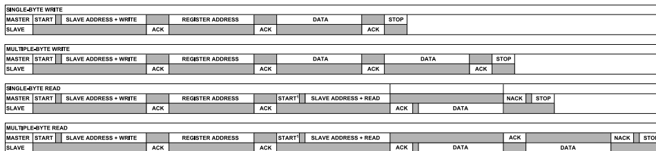
Figure 55. I 2 C Device Addressing (Read from Data Registers)
