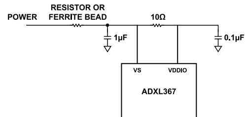
Figure 61. Recommended Decoupling Schematics for Single Supply
