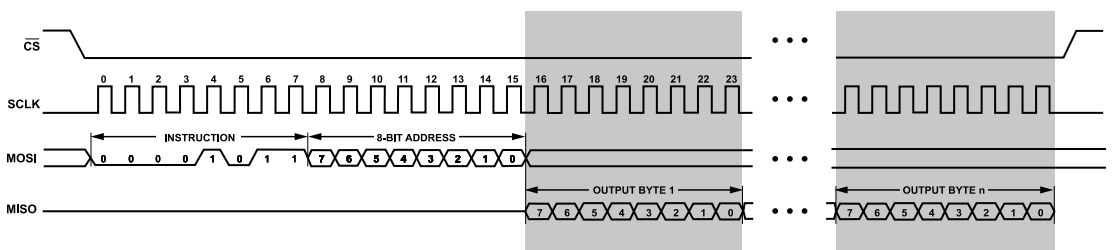
Figure 4. Burst Read
