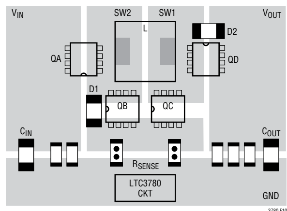
Figure 10. Switches Layout
