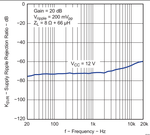
Figure 28. Supply Ripple Rejection Ratio vs Frequency (BTL)
