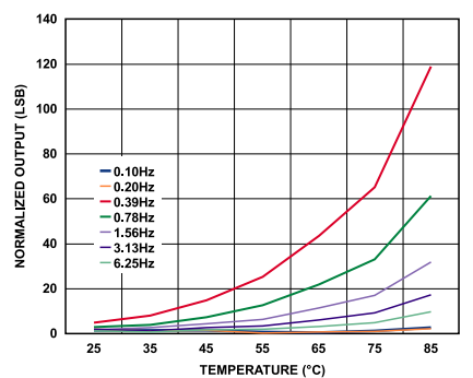
Figure 55. Typical Y-Axis Output vs. Temperature at Lower Data Rates, Normalized to 100 Hz Output Data Rate, V_S = 2.5 V
